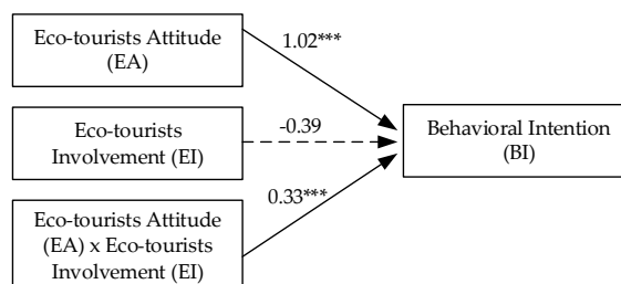
Figure 4: Path analysis of Model B.
