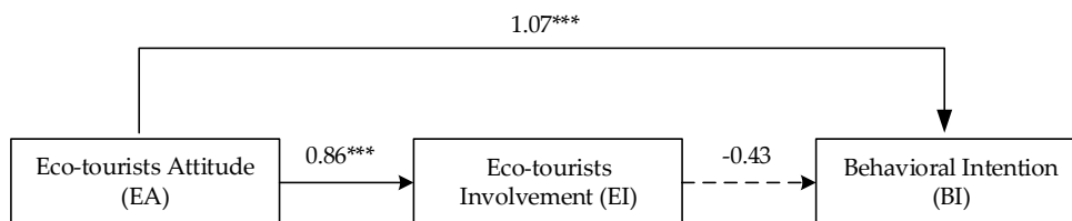
Figure 3: Path analysis of Model A.
