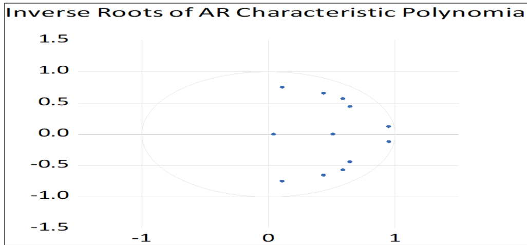
Figure 3: The dispersion shape for testing the stability of the overall model for the variables of the Iraqi National Bank.
